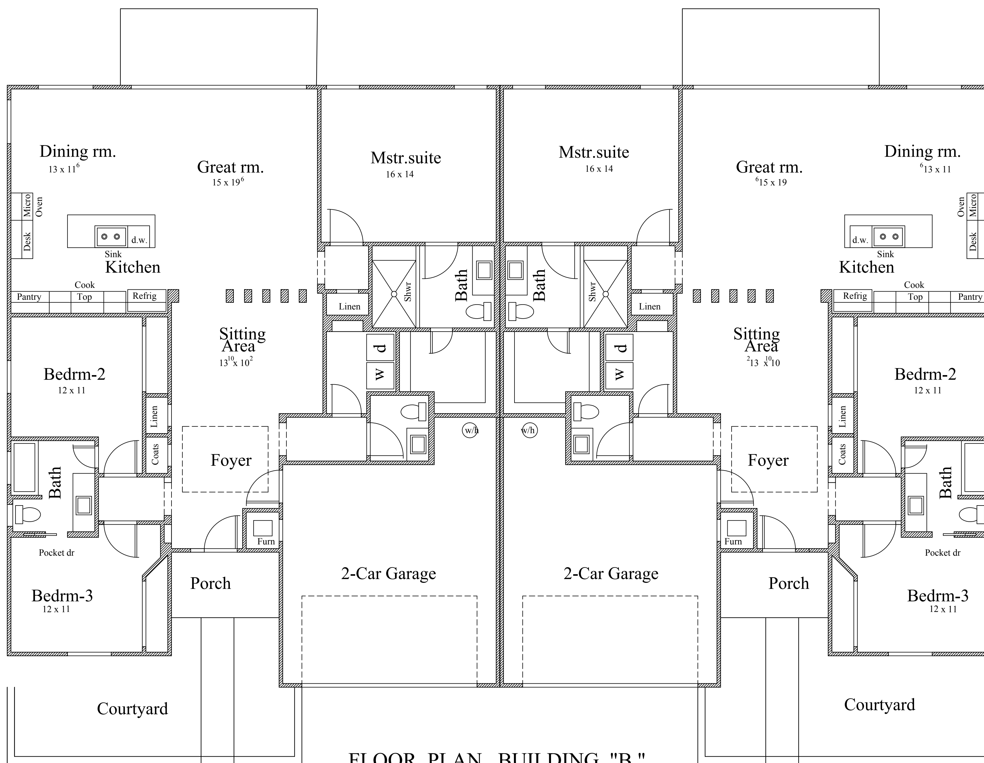
FLOOR PLAN BUILDING "B "
